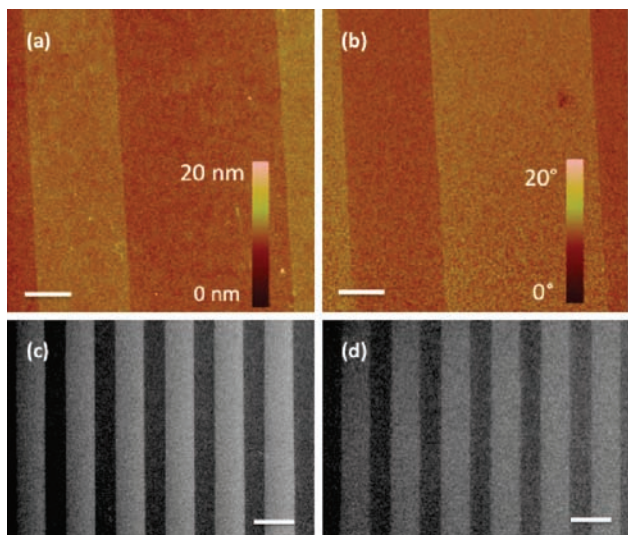
Figure 3. Characterization of P-selectin patterned substrates for cell rolling. AFM images of 10- \mu\text{m} -wide P-selectin lines separated by 15- \mu\text{m} -wide PEG bands (after step 2), displaying the contrast between P-selectin and PEG regions in (a) height and (b) phase, respectively. The phase image indicates a difference between the mechanical properties of the surface in the two regions. SEM images of surfaces (c) after PEG printing (step 1) and (d) after P-selectin adsorption (step 2), respectively, showing patterning uniformity (with brighter areas corresponding to PEG regions). Scale bars are (a, b) 5 \mu\text{m} and (c, d) 100 \mu\text{m} .
