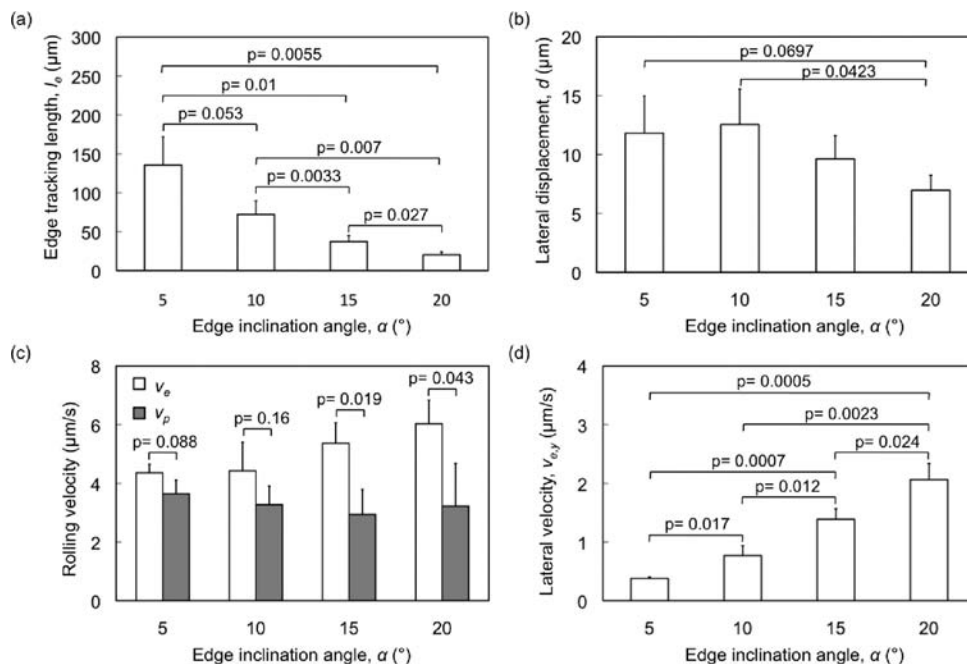
Figure 5. Effect of edge inclination angle \alpha on the rolling behavior of HL60 cells at a fluid shear stress magnitude of 0.5 \text{ dyn/cm}^2 and P-selectin incubation concentration of 15 \mu\text{g/mL} . Variation of the (a) edge tracking length, l_e ; (b) lateral displacement, d ; (c) rolling velocities, v_p and v_e , within the P-selectin lines and on the edge, respectively; and (d) lateral velocity, v_{e,y} , which is a component of the edge rolling velocity in the direction of lateral displacement. Error bars represent one standard deviation, where n = 3 replicate experiments for each condition.
