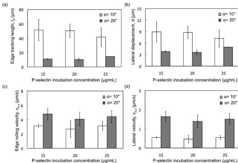
Figure 7. Effect of P-selectin incubation concentration on the rolling behavior of HL60 cells at a shear stress of 0.5 \text{ dyn/cm}^2 . Variation of the (a) edge tracking length, (b) lateral displacement, (c) edge rolling velocity, and (d) lateral velocity with P-selectin incubation concentration at edge inclination angles of \alpha = 10 and 20^\circ .
