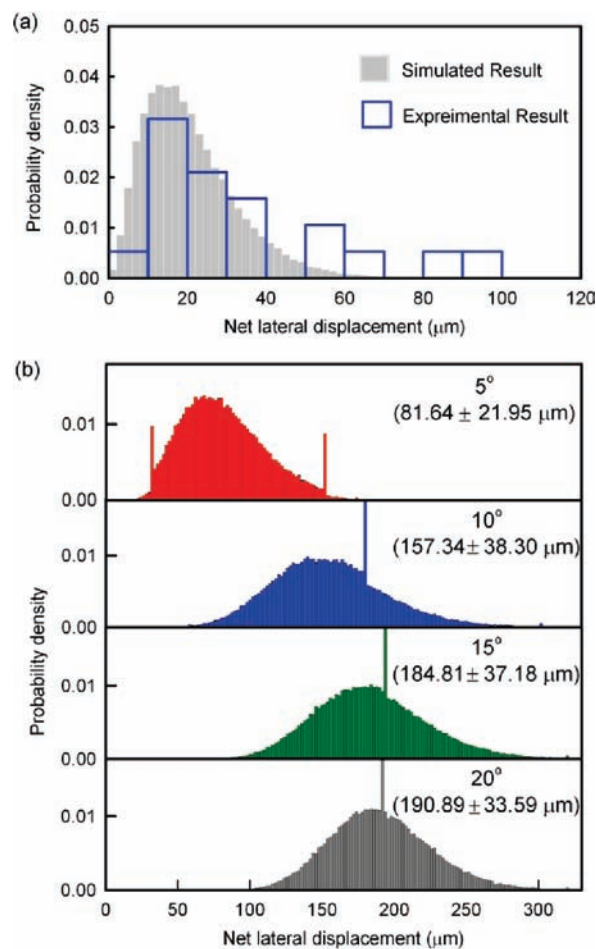
Figure 9. (a) Probability distribution of net lateral displacement of HL-60 cells after rolling on three consecutive lines of P-selectin patterns as obtained from Monte Carlo simulations (shaded area) and experimental observations. \alpha = 20^\circ (shear stress = 0.5 \text{ dyn/cm}^2 ). (b) Prediction of the downstream distribution of HL60 cells rolling on patterned P-selectin in a separation device. HL60 cells are introduced at a single location and travel a distance of 1 cm in the downstream direction, interacting with a substrate patterned with P-selectin lines of 50 \mu\text{m} width separated by 70 \mu\text{m} PEG gaps. A net lateral displacement of 10^5 cells was calculated by assuming that detachment on the edge was governed by a Poisson process with parameters as obtained earlier by fitting to experimental data at a shear stress of 0.5 \text{ dyn/cm}^2 . The numbers in parentheses denote the net lateral displacement and standard deviation. The “spikes” appear at the position where the edges intersect the 1 cm downstream position. (The full extent of the spikes is not shown.)
