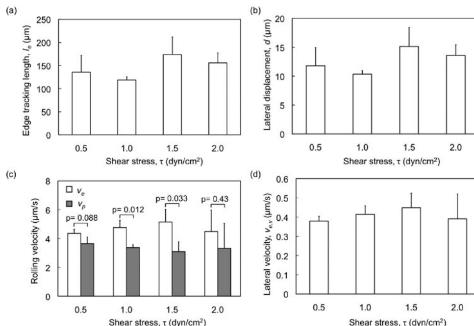
Figure 6. Effect of shear stress \tau on the rolling behavior of HL60 cells at an edge inclination angle of 5°. Variation of the (a) edge tracking length, l_e ; (b) lateral displacement, d ; (c) rolling velocities, v_p and v_e , within the P-selectin lines and on the edge, respectively; and (d) lateral rolling velocity, v_{e,y} . Error bars represent one standard deviation, where n = 3 replicate experiments for each condition.
