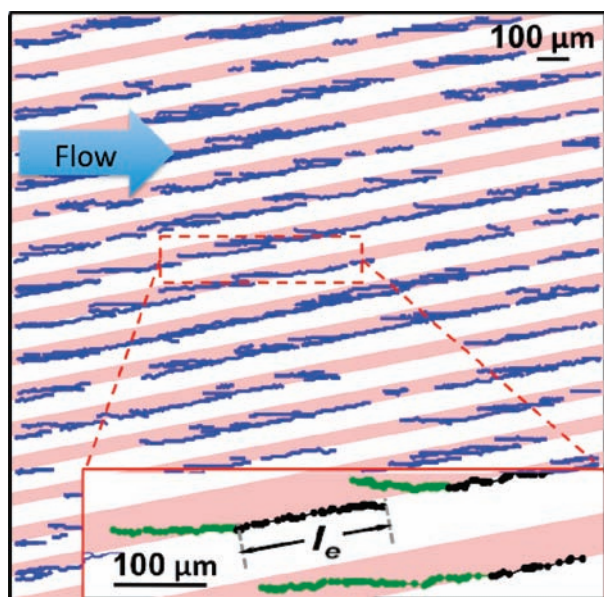
Figure 4. Tracks of HL60 cells rolling (blue lines) on P-selectin lines (pink) were obtained by analyzing 300 images acquired at 1 fps using a customized Matlab code. The edge inclination angle was 10°, and the shear stress was 0.5 dyn/cm 2 . The inset shows a track corresponding to a cell that first rolled inside the P-selectin line (green) in the direction of fluid flow and then tracked along the edge (black).
