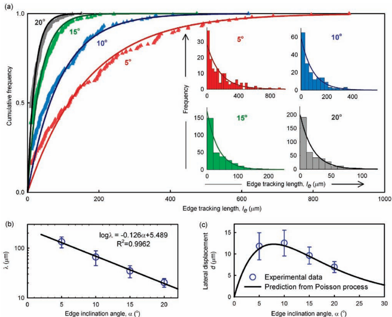
Figure 8. Detachment of cells rolling along an edge can be described by a Poisson distribution. (a) Cumulative distribution function of edge tracking lengths l_e (filled triangles) fitted to a Poisson distribution described by eq 1 (solid lines). Insets show the frequency distribution of the experimentally measured edge tracking lengths, along with that predicted by the Poisson distribution fit to the CDF (solid lines). Colors indicate different inclination angles \alpha of the receptor pattern. Representative results are shown for only one experiment for each \alpha . (b) Variation of the average value of \lambda with the edge inclination angle can be described by a linear fit to a semilog plot (solid line). (c) Variation with the edge inclination angle of the average value of the lateral displacement (solid line) obtained from the empirical fit shown in plot b along with the experimental results (open circles). Error bars in plots b and c represent one standard deviation. The shear stress is 0.5 \text{ dyn/cm}^2 .
